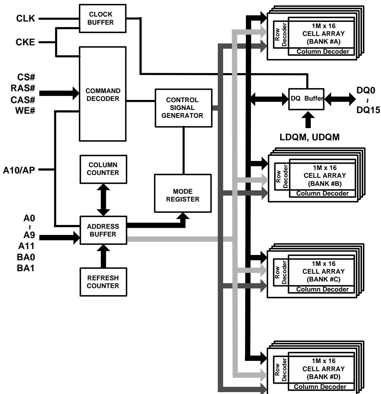
Figure 2. Block Diagram
