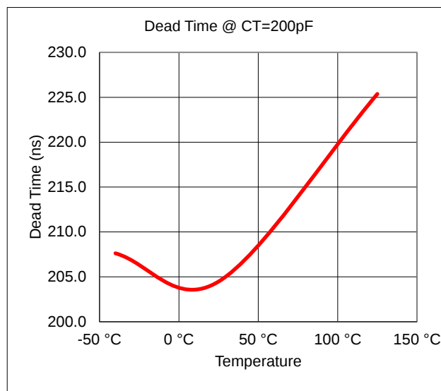
Figure 14: Dead-Time vs Temperature
