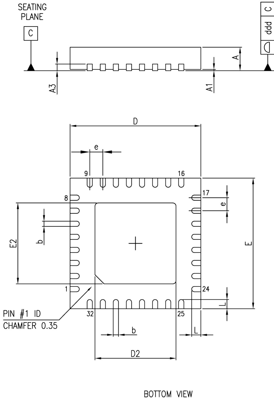
Figure 35. VFQFPN32 (5 x 5 x 1 pitch, 0.5 mm) package outline (BlueNRG-132S)
