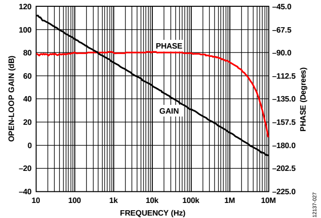
Figure 27. Open-Loop Gain and Phase vs. Frequency
