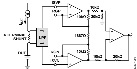
Figure 50. 4-Terminal Shunt Resistor Connected to the Current Sense IA
