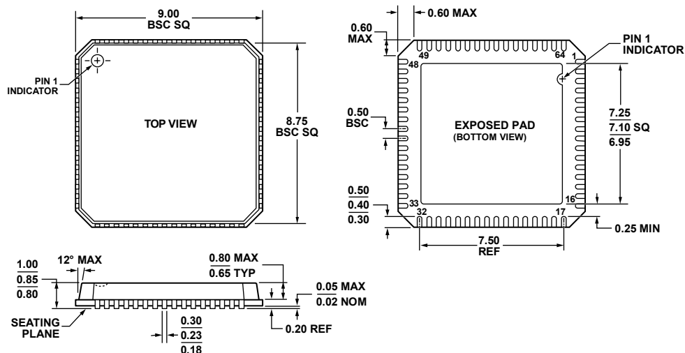
Figure 101. 64-Lead Lead Frame Chip Scale Package [LFCSP_VQ]
