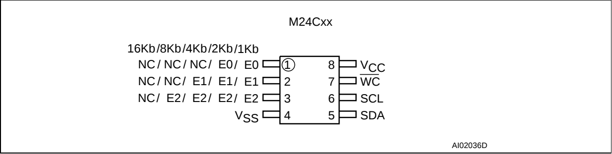
Figure 2C. Standard-TSSOP Connections
