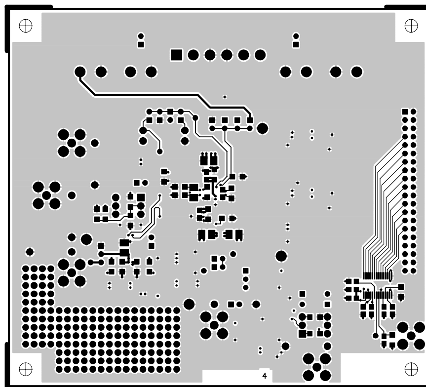
Figure 43. TSSOP Evaluation Board Layout, Secondary Side
