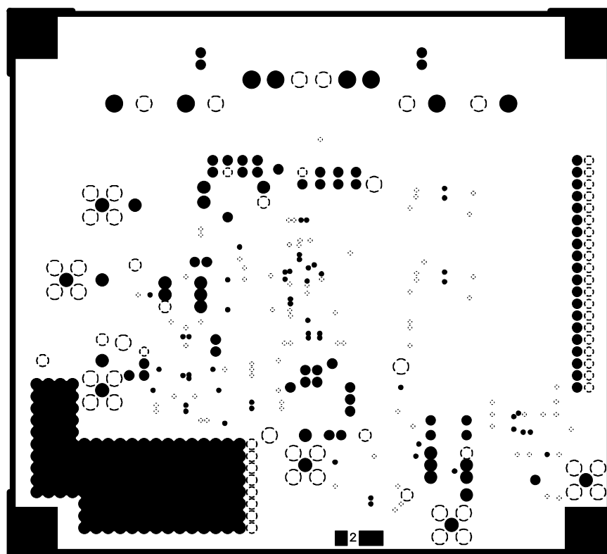
Figure 44. TSSOP Evaluation Board Layout, Ground Plane
