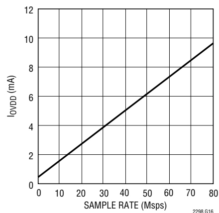
LTC2298: I_{VDD} vs Sample Rate, 5MHz Sine Wave Input, -1dB, O_{VDD} = 1.8\text{V}
