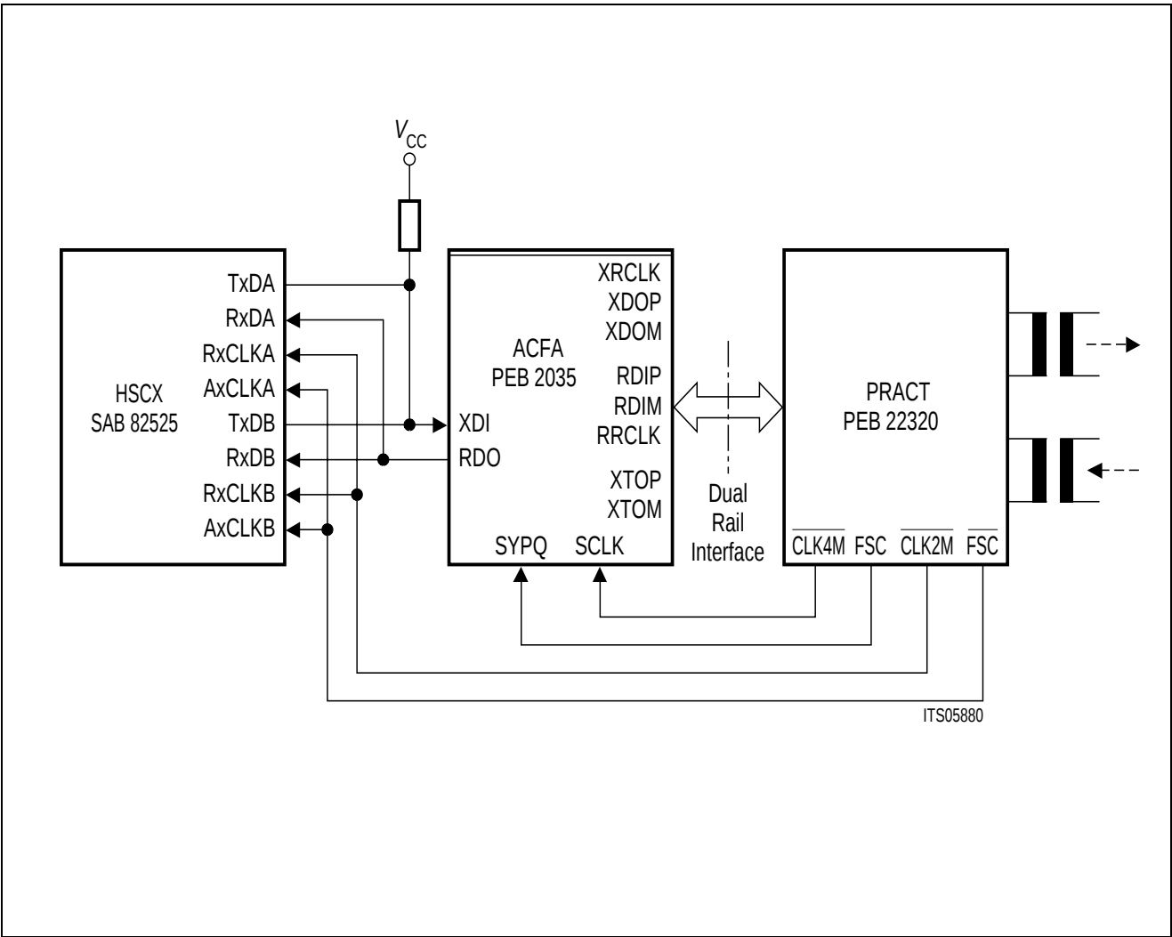
HSCX System Integration for Primary Rate Interface T1/E1 Siemens System Interface (ACFA/PRACT)
