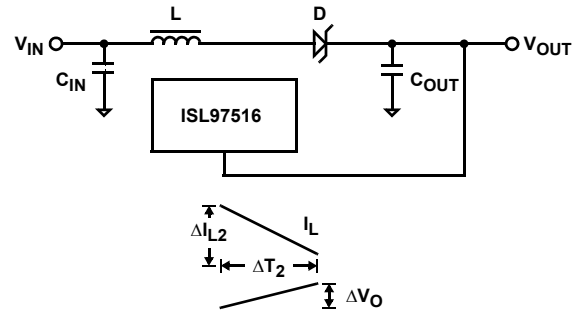
FIGURE 13. BOOST CONVERTER - CYCLE 2, POWER SWITCH OPEN
