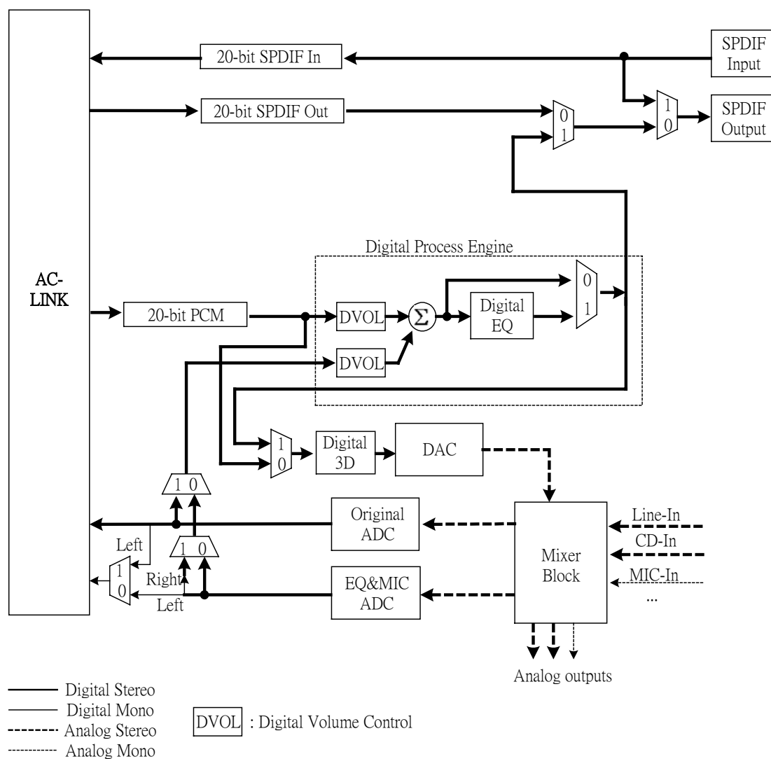
Figure. Digial Data Path Diagram
