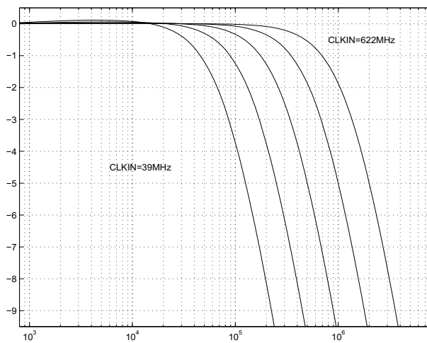
Figure 4. PLL Jitter Transfer Functions, MULTSEL = 0 (MULTOUT = 600–668 MHz)
