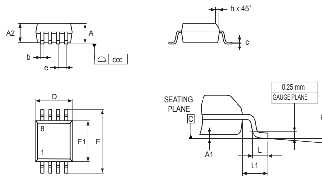
Figure 22. SO8N – Outline
