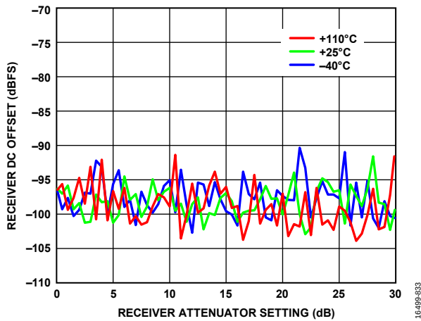
Figure 331. Receiver DC Offset vs. Receiver Attenuator Setting, LO = 4600 MHz
