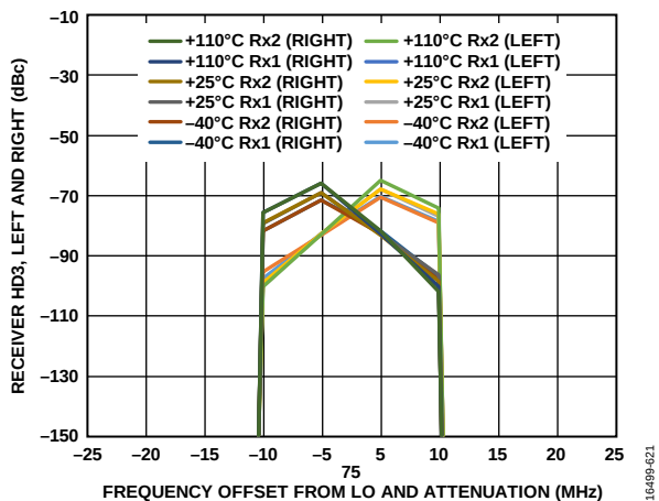
Figure 118. Receiver HD3 Left and Right vs. Frequency Offset from LO and Attenuation, Tone Level = -16 dBm at Attenuation = 0, LO = 75 MHz
