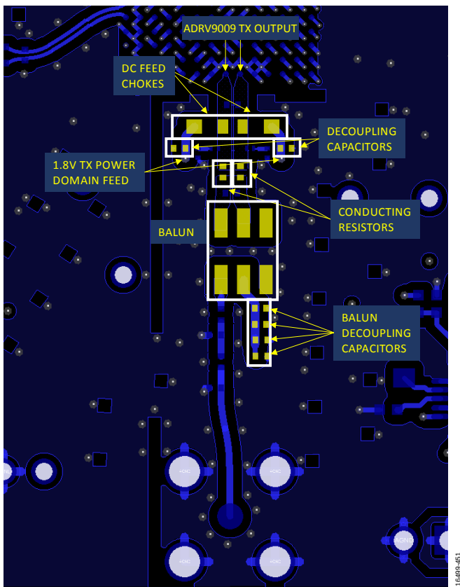
Figure 444. The Transmitter DC Chokes and Balun Feed Supply
