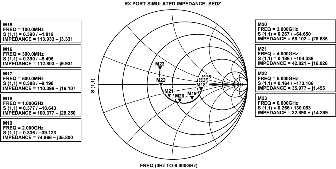
Figure 429. Receiver Input Impedance SEDZ
