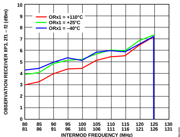
Figure 56. Observation Receiver IIP3, 2f_1 - f_2 vs. Intermod Frequency, LO = 75 MHz, Attenuation = 0 dB, Tones Separated By 1 MHz Swept Across Pass Band at -25 dBm Each
