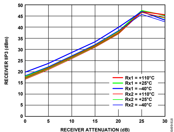
Figure 316. Receiver IIP3 vs. Receiver Attenuation, LO = 3600 MHz, Tone 1 = 3602 MHz, Tone 2 = 3692 MHz, -21 dBm Plus Attenuation
