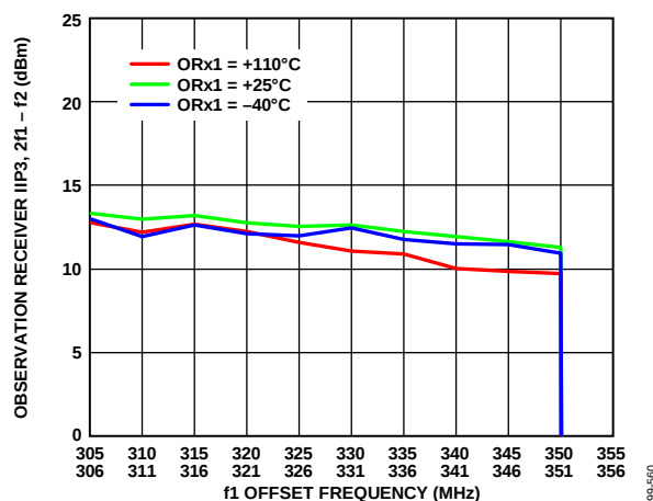
Figure 57. Observation Receiver IIP3, 2f_1 - f_2 vs. f_1 Offset Frequency, LO = 300 MHz, Attenuation = 0 dB, Tones Separated By 1 MHz Swept Across Pass Band at -25 dBm Each
