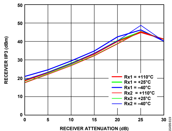
Figure 317. Receiver IIP3 vs. Receiver Attenuation, LO = 4600 MHz, Tone 1 = 4602 MHz, Tone 2 = 4692 MHz, -21 dBm Plus Attenuation
