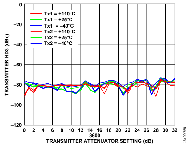
Figure 256. Transmitter HD3 vs. Transmitter Attenuator Setting, LO = 3600 MHz, Continuous Wave = -15 dBFS, Baseband Frequency = 10 MHz
