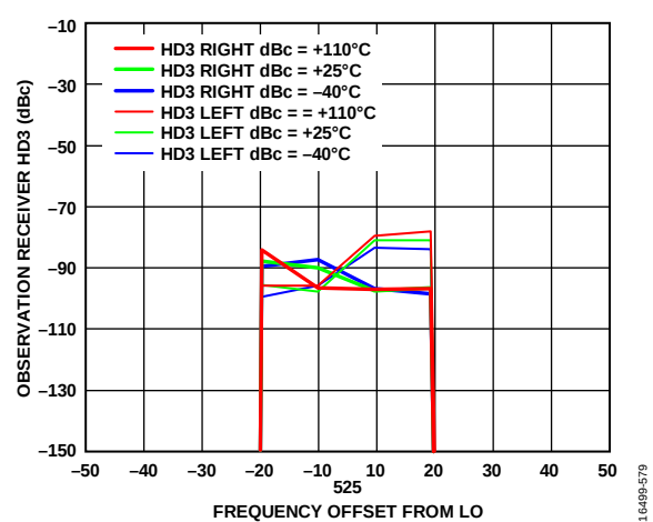
Figure 76. Observation Receiver HD3 Left and Right vs. Frequency Offset from LO, Tone Level -22 dBm at Attenuation = 0, LO = 525 MHz
