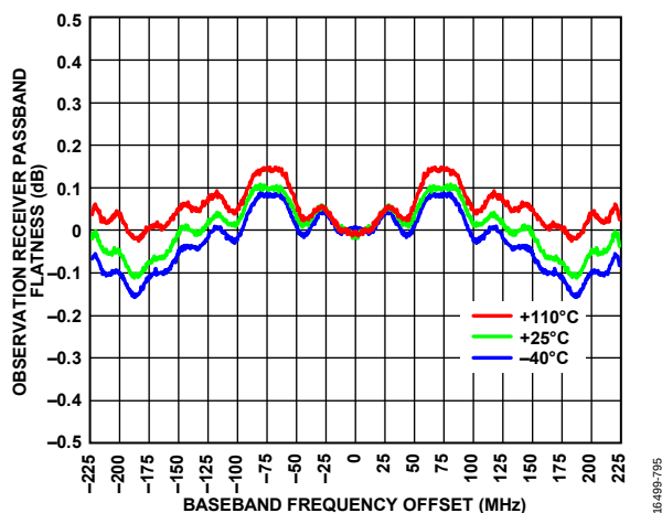
Figure 292. Observation Receiver Pass Band Flatness vs. Baseband Frequency Offset, LO = 4600 MHz
