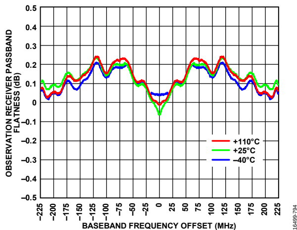
Figure 291. Observation Receiver Pass Band Flatness vs. Baseband Frequency Offset, LO = 3600 MHz
