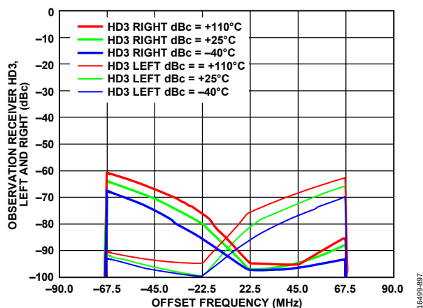
Figure 398. Observation Receiver HD3, Left and Right vs. Offset Frequency, LO = 5700 MHz, Tone Level = -20 dBm
