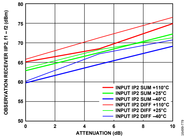
Figure 276. Observation Receiver IIP2, 2f_1 - f_2 vs. Attenuation, 4600 MHz, Tone 1 = 4602 MHz, Tone 2 = 4612 MHz at -22 dBm Plus Attenuation
