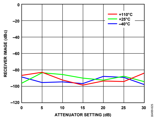
Figure 323. Receiver Image vs. Attenuator Setting, 200 MHz RF Bandwidth, Tracking Calibration Active, Sample Rate = 245.76 MSPS, LO = 4600 MHz, Baseband Frequency = 10 MHz
