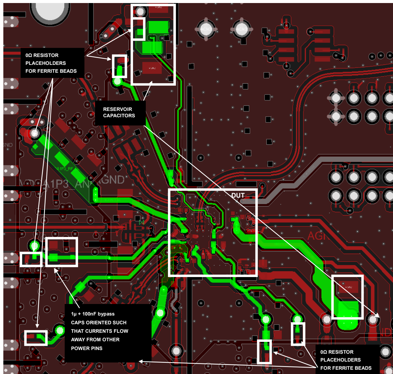
Figure 439. Placement Example of 0 \Omega Resistor Placeholders for Ferrite Beads, Reservoir and Bypass Capacitors on ADRV9009 Customer Card (Layers: 12 to Power and Bottom)
