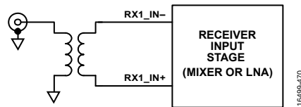
Figure 461. Differential Receiver Interface Using a Transformer
