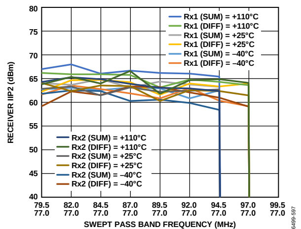
Figure 94. Receiver IIP2 Sum and Difference Across Bandwidth, 0 dB Receiver Attenuation, LO = 75 MHz, Tone 1 = 77 MHz, Tone 2 Swept, -23.5 dBm Each
