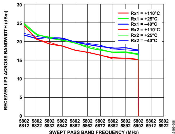
Figure 409. Receiver IIP3 Across Bandwidth vs. Swept Pass Band Frequency, Receiver Attenuation = 0 dB, LO = 5800 MHz, Tone 1 = 5802 MHz, Tone 2 Swept Across Pass Band, -21 dBm Each
