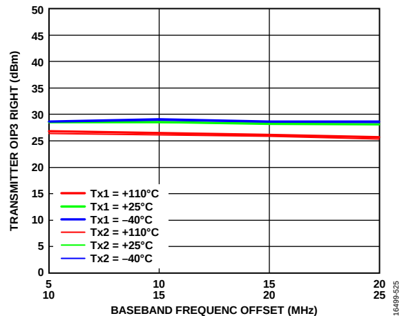
Figure 22. Transmitter OIP3 Right vs. Baseband Tone Pair Swept Across Pass Band, LO = 75 MHz, Total RMS Power = -12 dBFS, 4 dB Transmitter Attenuation
