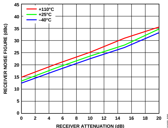
Figure 197. Receiver Noise Figure vs. Receiver Attenuation, LO = 2850 MHz, 200 MHz Bandwidth, Sample Rate = 245.76 MSPS, Integration Bandwidth = 500 kHz to 100 MHz
