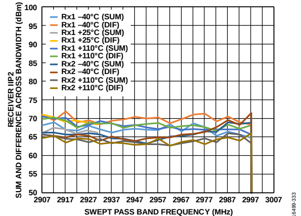
Figure 210. Receiver IIP2 Sum and Difference Across Bandwidth vs. Swept Pass Band Frequency, Receiver Attenuation = 0 dB, LO = 2900 MHz, Tone 1 = 2902 MHz, Tone 2 Swept, -21 dBm Each
