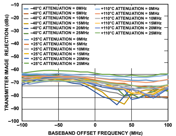
Figure 243. Transmitter Image Rejection Across Large Signal Bandwidth vs. Baseband Offset Frequency and Attenuation, QEC Trained with Three Tones (Tracking On), Total Combined Power = -6 dBFS, Correction Then Frozen (Tracking Turned Off), Continuous Wave Tone Swept Across Large Signal Bandwidth, LO = 4600 MHz
