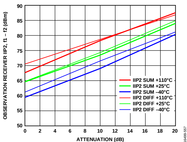
Figure 54. Observation Receiver IIP2, f_1 - f_2 vs. Attenuation, LO = 300 MHz, Tone 1 = 302 MHz, Tone 2 = 322 MHz at -25 dBm Plus Attenuation
