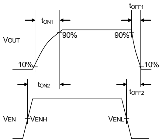
Figure 2. Timing Diagram(BD2068FJ-M)
