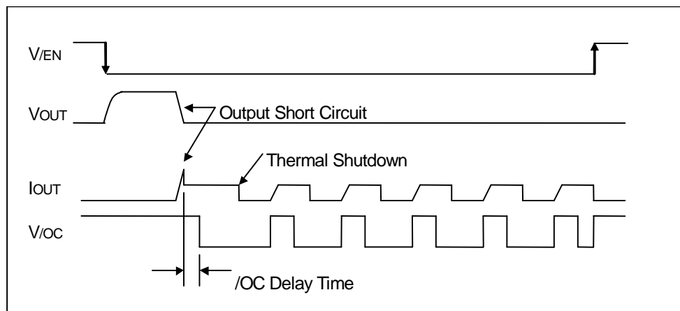
Figure 39. Over Current Detection, Thermal Shutdown Timing (BD2069FJ-M)
