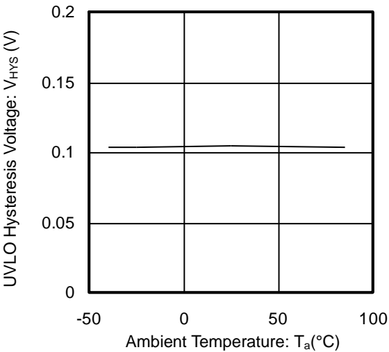
Figure 29. UVLO Hysteresis Voltage vs Ambient Temperature
