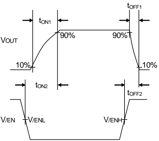
Figure 3. Timing Diagram(BD2069FJ-M)
