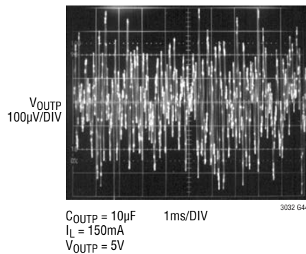
OUTP 10Hz to 100kHz Output Noise, C_BYPP = 0
