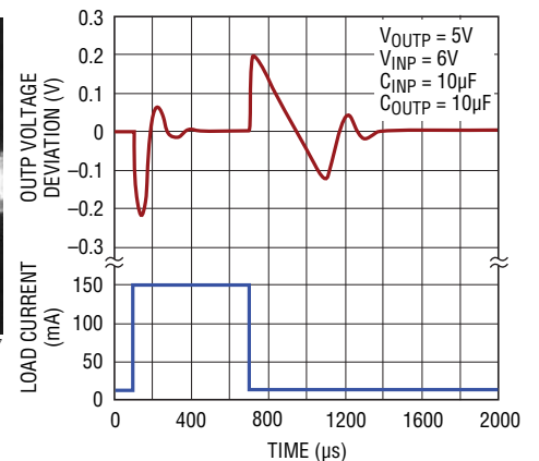
OUTP Transient Response, C_BYPP = 0
