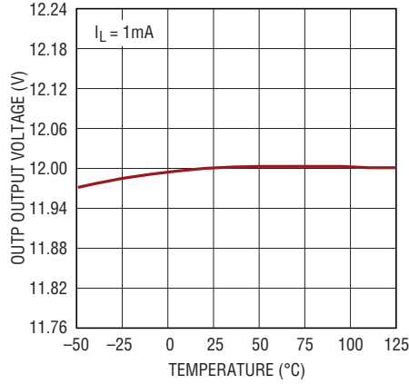
LT3032-12 OUTP Output Voltage
