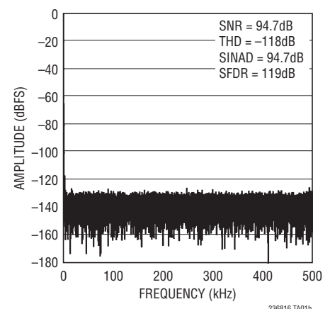
32k Point FFT f_{\text{S}} = 1\text{Msps} , f_{\text{IN}} = 2\text{kHz}
