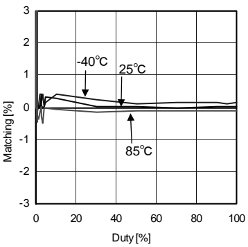
Fig 15. LED Current Matching
