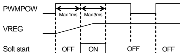
Fig.20 Soft start
