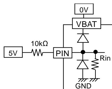
Fig.29 Example of application at control signal voltage > VBAT voltage
