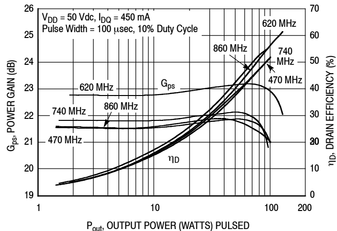
Figure 23. Pulsed Power Gain and Drain Efficiency versus Output Power (Broadband Reference Circuit)
