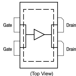
Figure 1. Pin Connections
