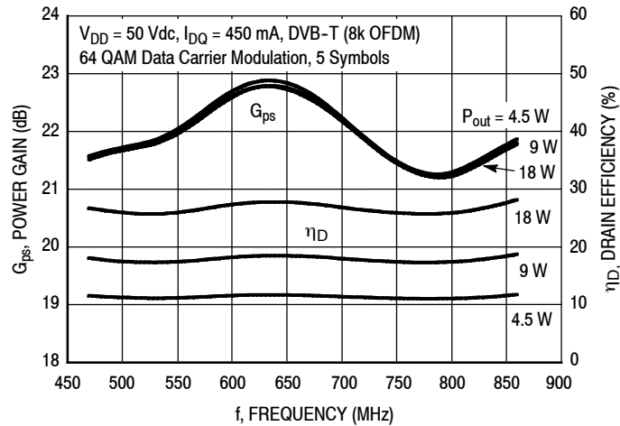
Figure 21. Single-Carrier DVB-T (8k OFDM) Power Gain and Drain Efficiency versus Frequency (Broadband Reference Circuit)
