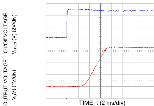
Figure 15. Typical Start-Up Using Remote On/Off with Low-ESR external capacitors ( V_{in} = 5.5\text{ Vdc} , V_o = 3.3\text{ Vdc} , I_o = 16.0\text{ A} , C_o = 1050\text{ }\mu\text{F} ).
