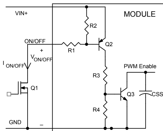
Figure 28. Remote On/Off Implementation.
