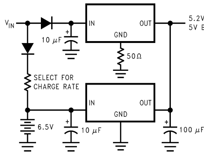
Battery Backup Regulated Supply
