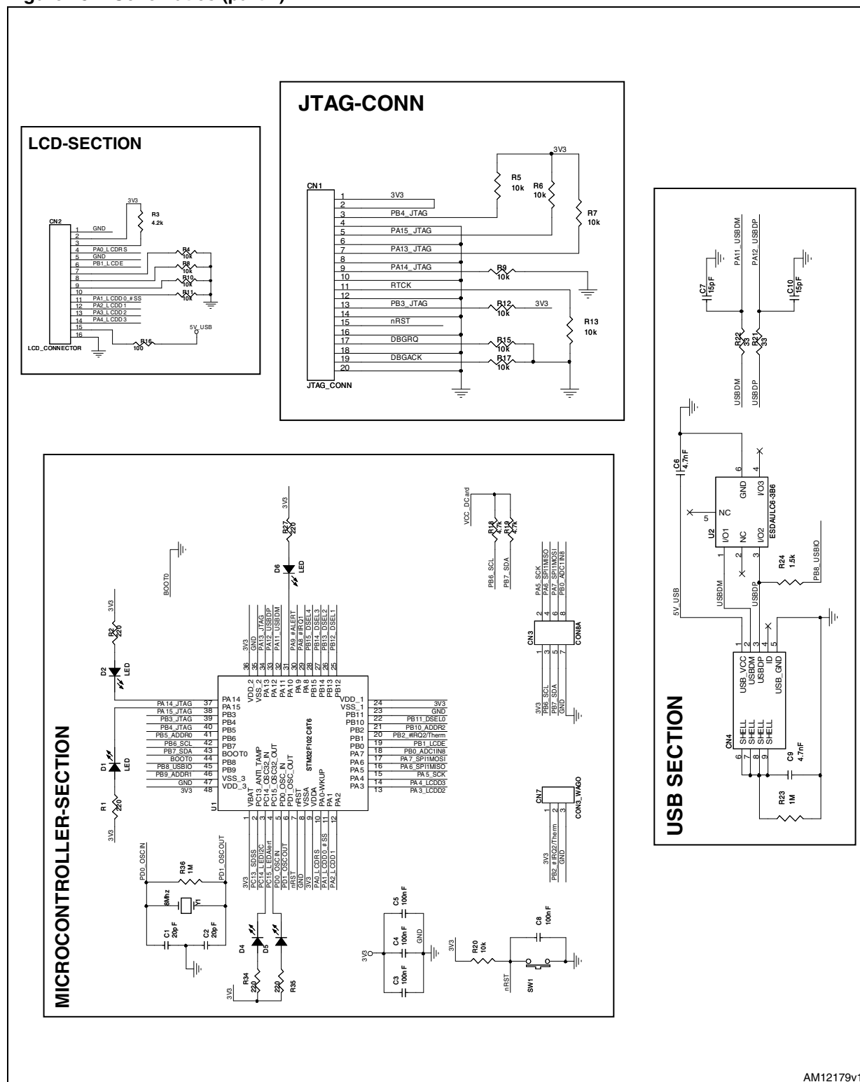
Figure 25. Schematics (part 1)
