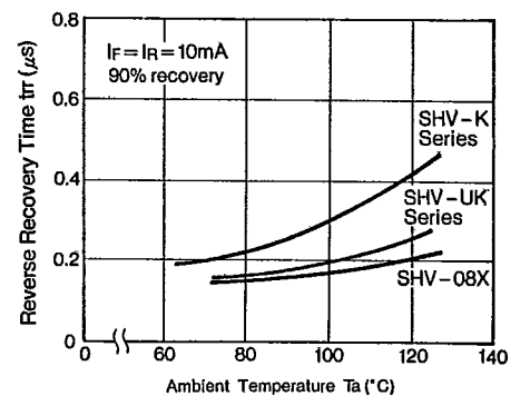
trr - t a Characteristics
