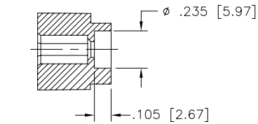
SECTION U-U
