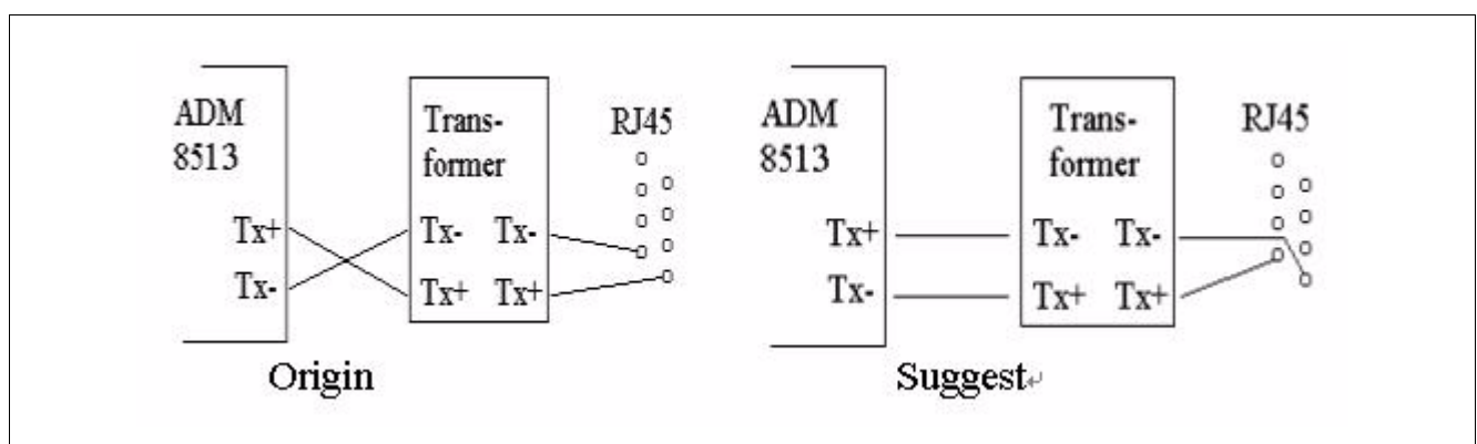
Figure 10 Trace Routing 2
