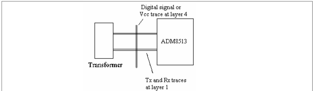
Figure 11 Trace Routing 3
