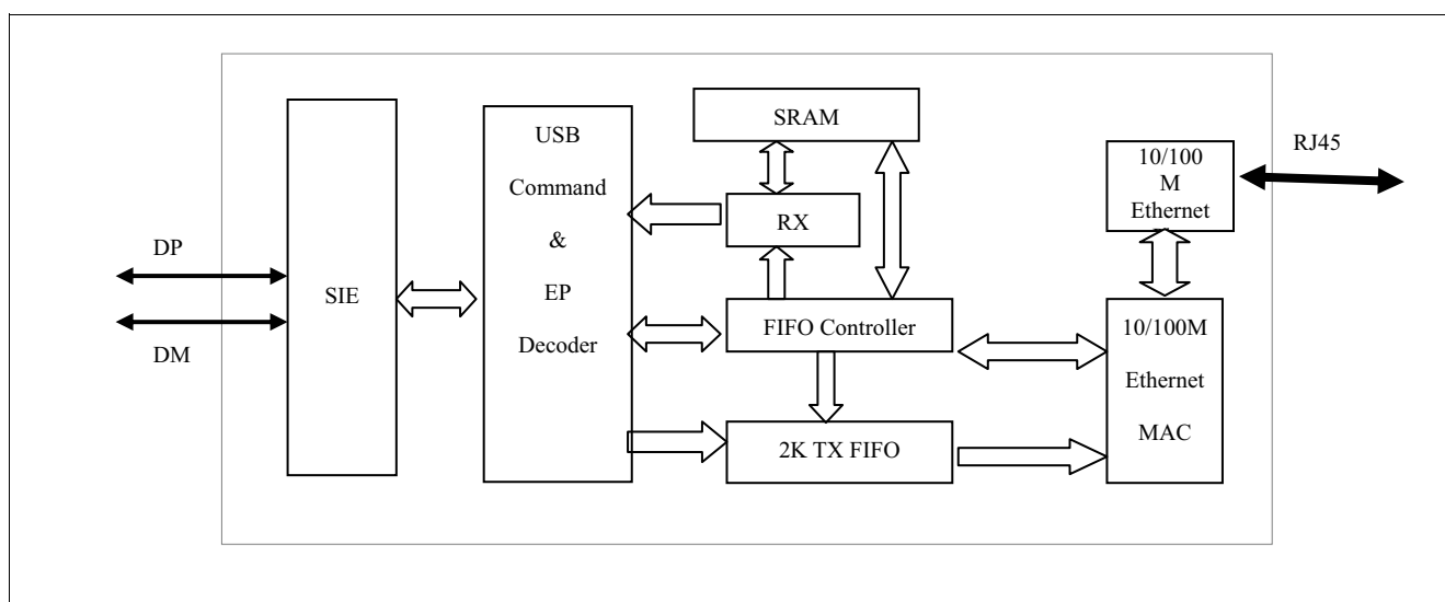
Figure 2 Block Diagram
