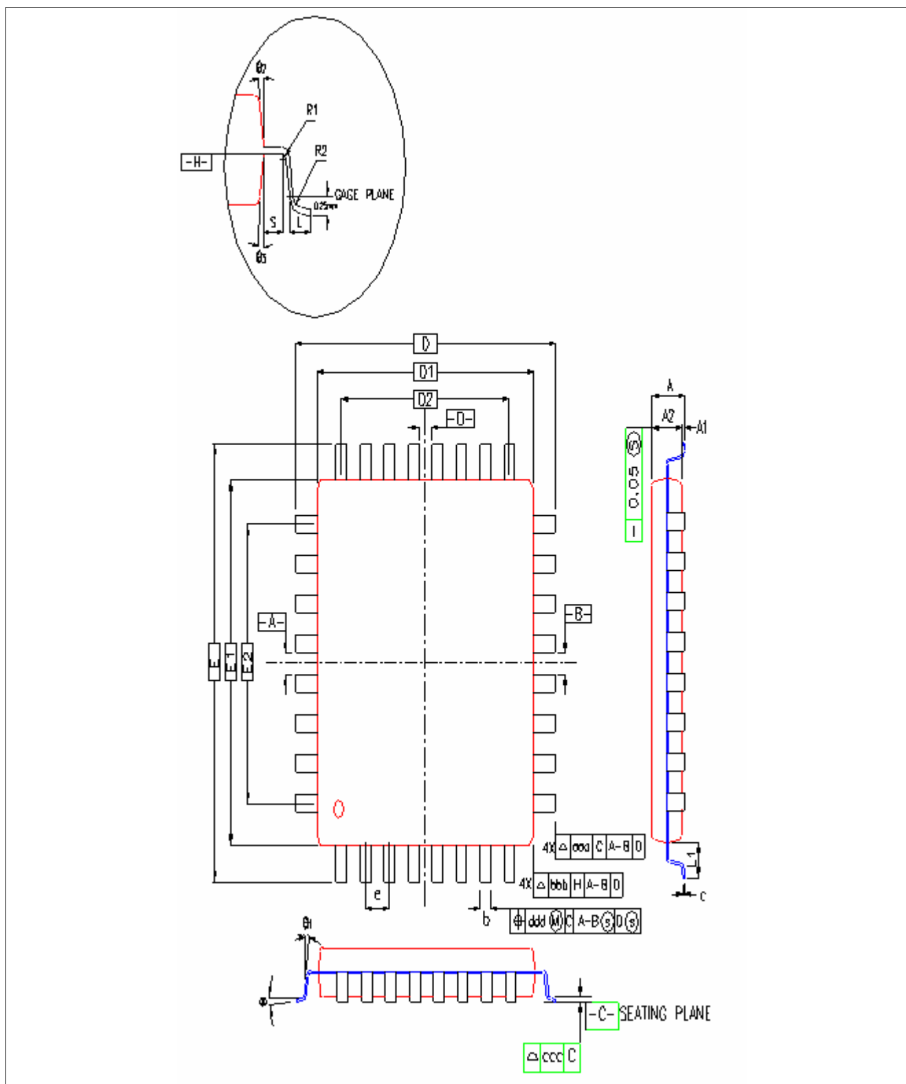
Figure 6 Package
