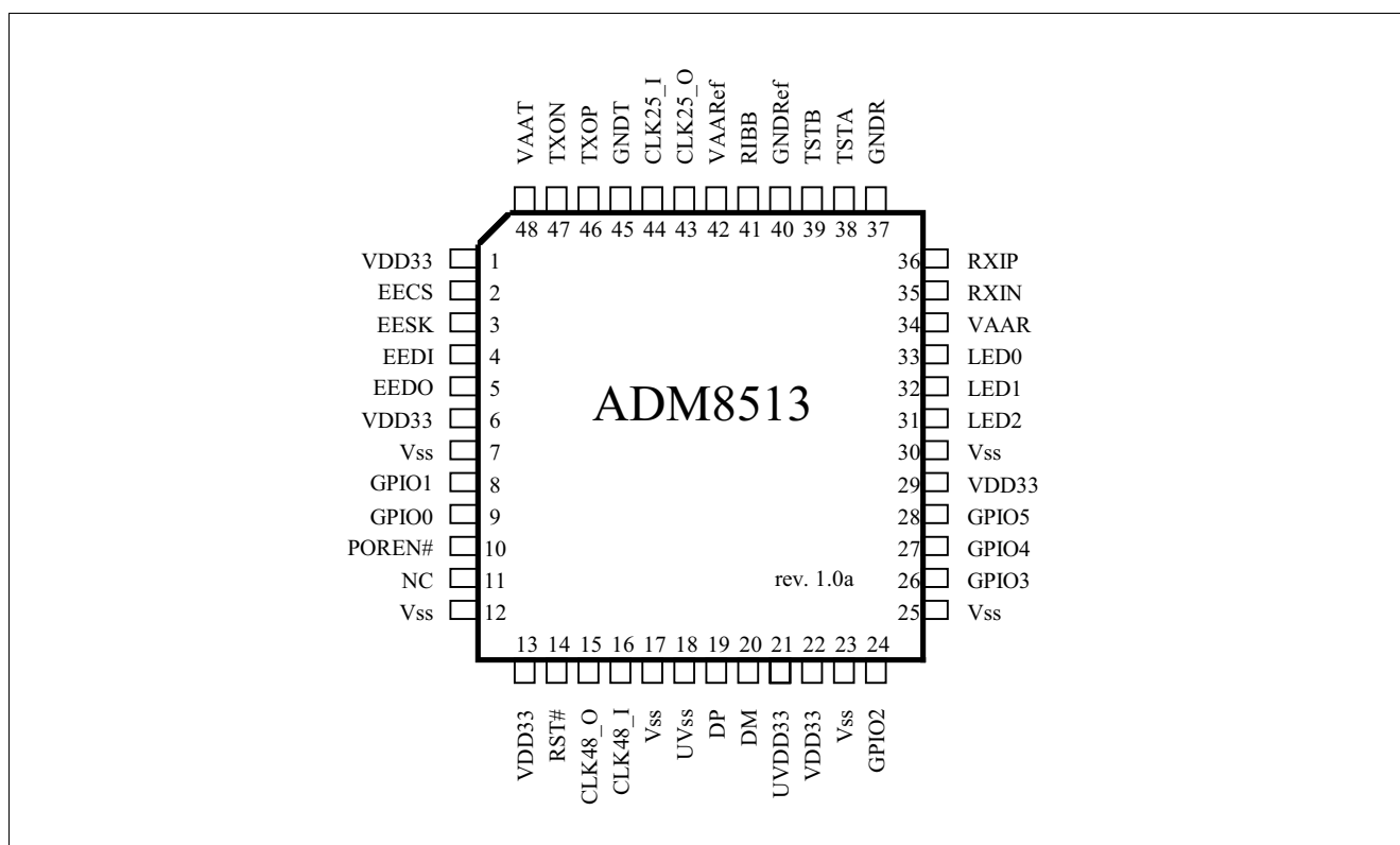
Figure 1 Pin Diagram
