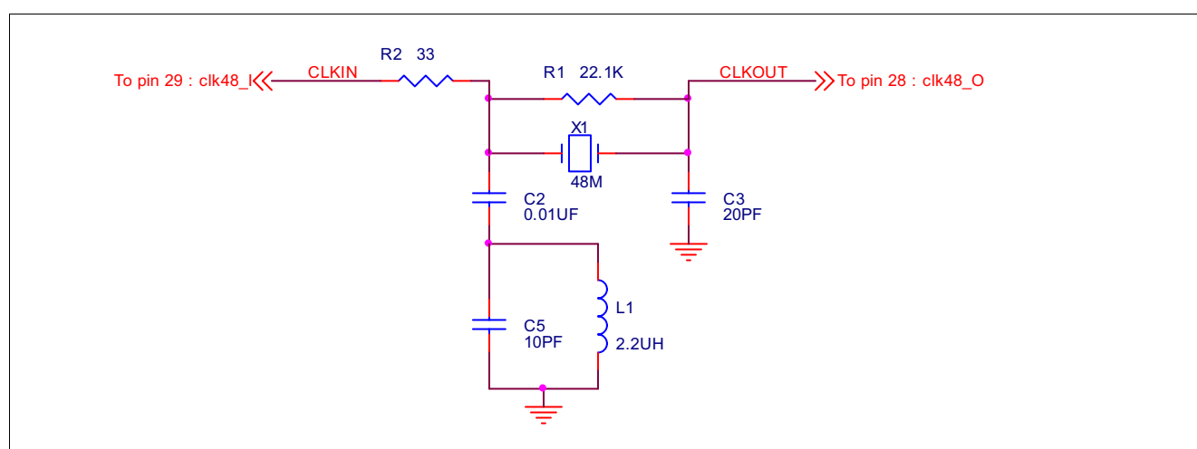
Figure 7 Placement 1
