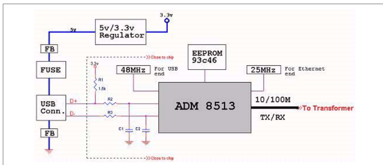
Figure 8 Placement 2
