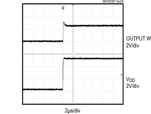
MAX5387 POWER-ON WIPER TRANSIENT (CODE 0 TO 128)
