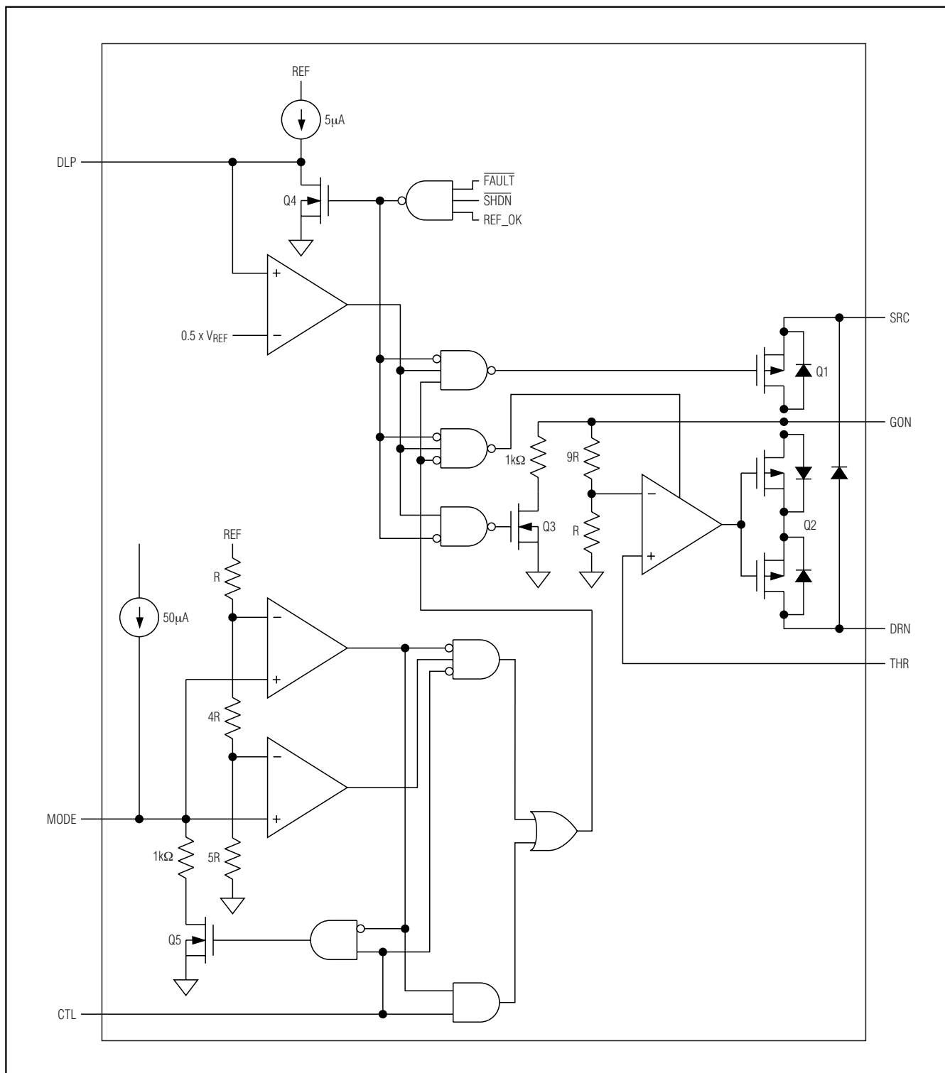
Figure 4. Switch Control
