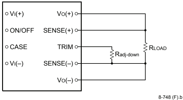
Figure 21. Circuit Configuration to Decrease Output Voltage
