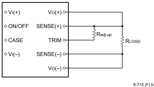
Figure 22. Circuit Configuration to Increase Output Voltage
