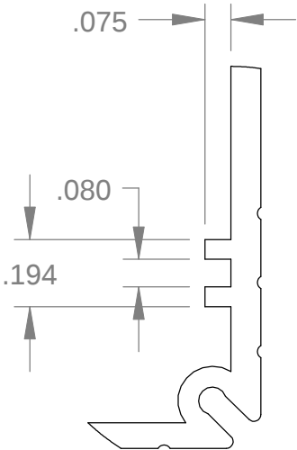
DETAIL C
