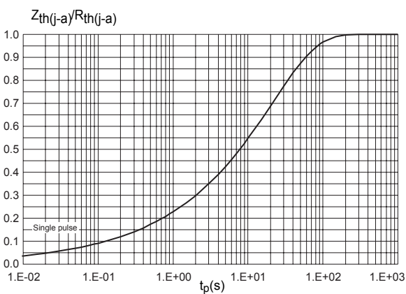
Figure 5. Relative variation of thermal impedance junction to ambient versus pulse duration (SMB)
