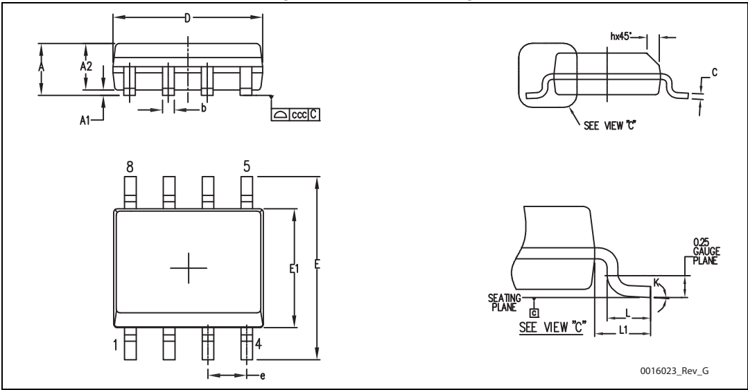
Figure 14. SO-8 drawings
