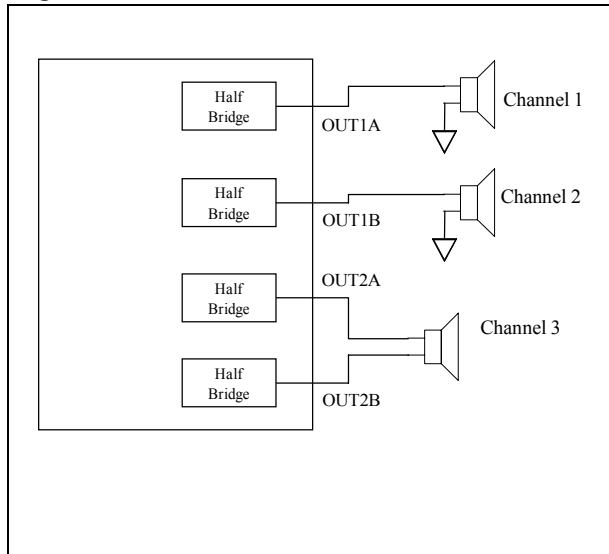
Figure 13. OCFG = 11
