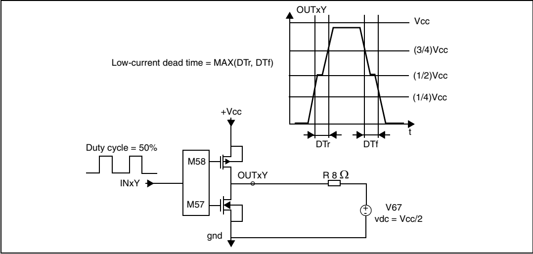
Figure 4. Test circuit 1
