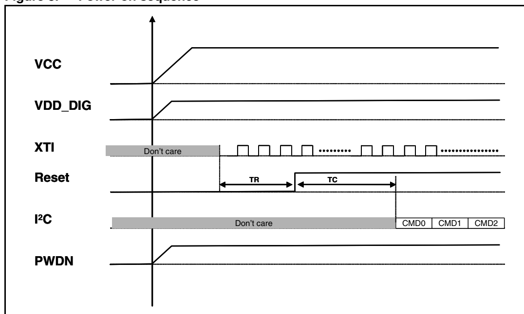
Figure 3. Power-on sequence
