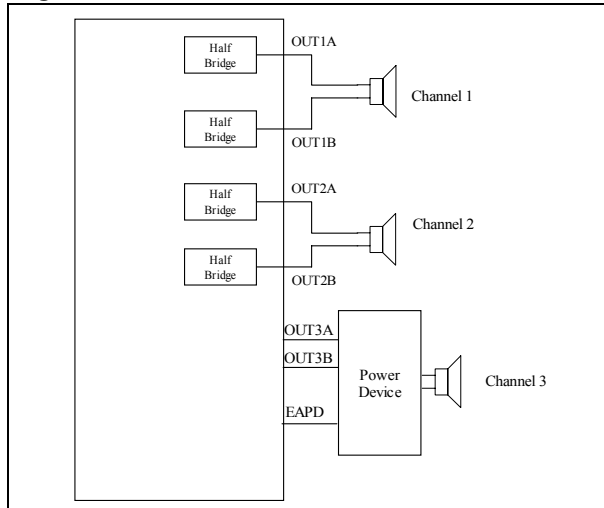
Figure 12. OCFG = 10
