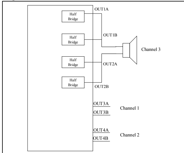
Figure 13. OCFG = 11
