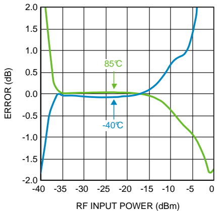
Figure 21. 10 dB Power Step Error vs. RF Input Power at 900 MHz
