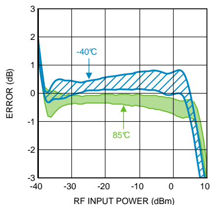
Figure 13. Log Conformance Error (50 Units) vs. RF Input Power at 50 MHz
