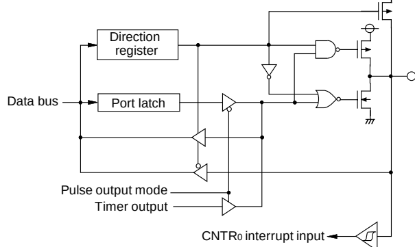
(11) Port P54
