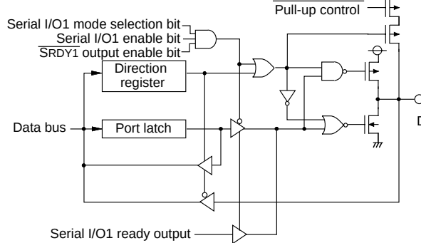
(8) Port P47
