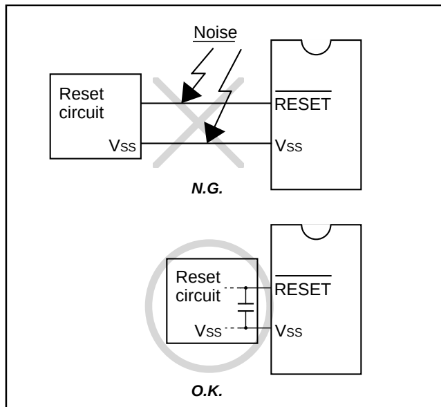
Fig. 63 Wiring for the RESET pin
