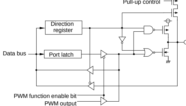
(10) Ports P50,P51
