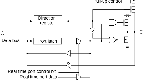
(9) Ports P52,P53
