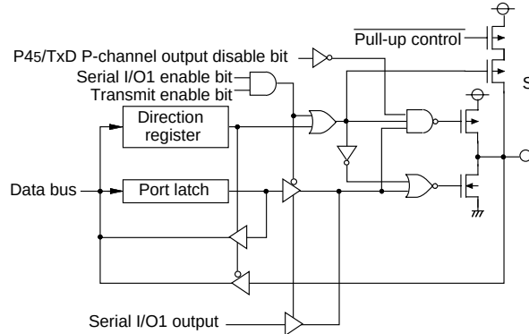
(6) Port P45
