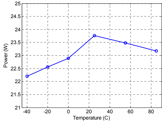
Power vs. Temperature, 5400 MHz, 3dB Compression V_{DS}=28V , I_{DQ}=50mA ; Pulse: 100 \mu s , 20%
