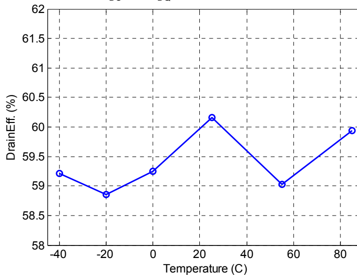
Drain Efficiency vs. Temperature, 5400 MHz, 3dB Compression V_{DS}=28V , I_{DQ}=50mA ; Pulse: 100 \mu s , 20%
