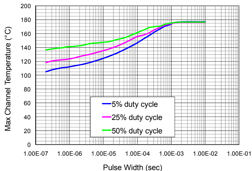
Max Channel Temperature Tbase = 85 °C, Pdis = 3 w/mm
