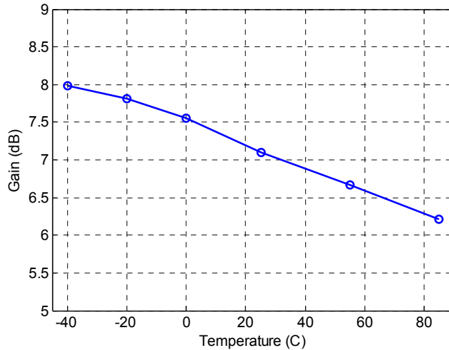
Gain vs. Temperature, 5400 MHz, 3dB Compression V_{DS}=28V , I_{DQ}=50mA ; Pulse: 100 \mu s , 20%
