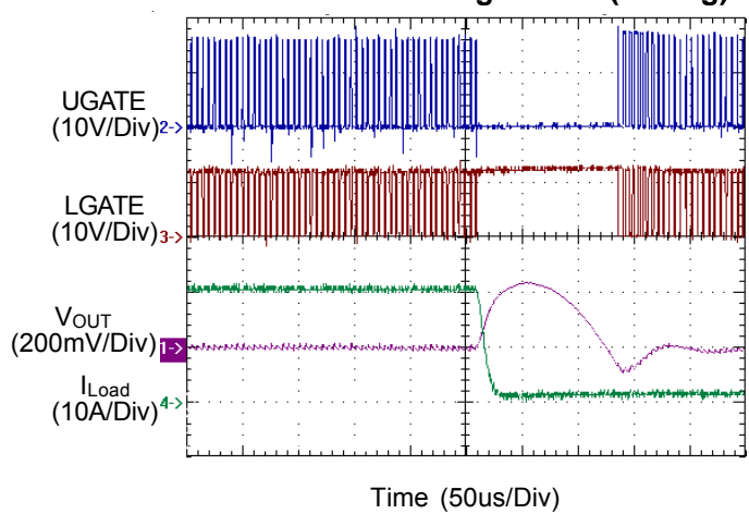
Load Transient Regulation (Falling)
