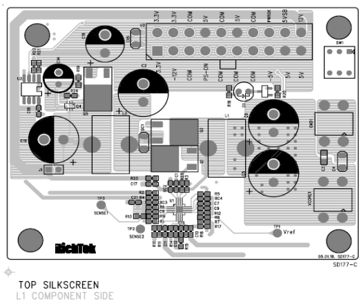
Figure 13. Component Side
