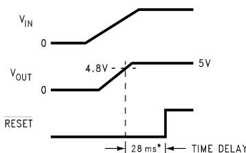
Figure 39. Timing Diagram for Timed Power-On Reset
