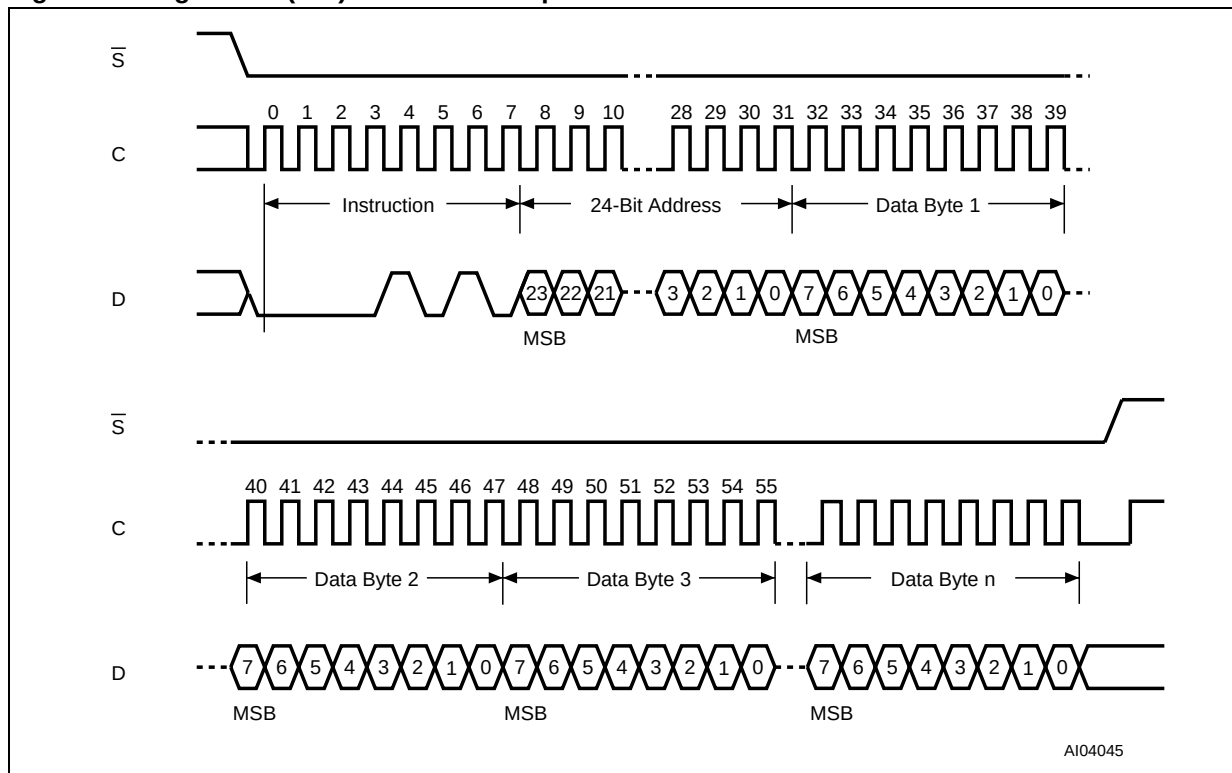
Figure 14. Page Write (PW) Instruction Sequence
