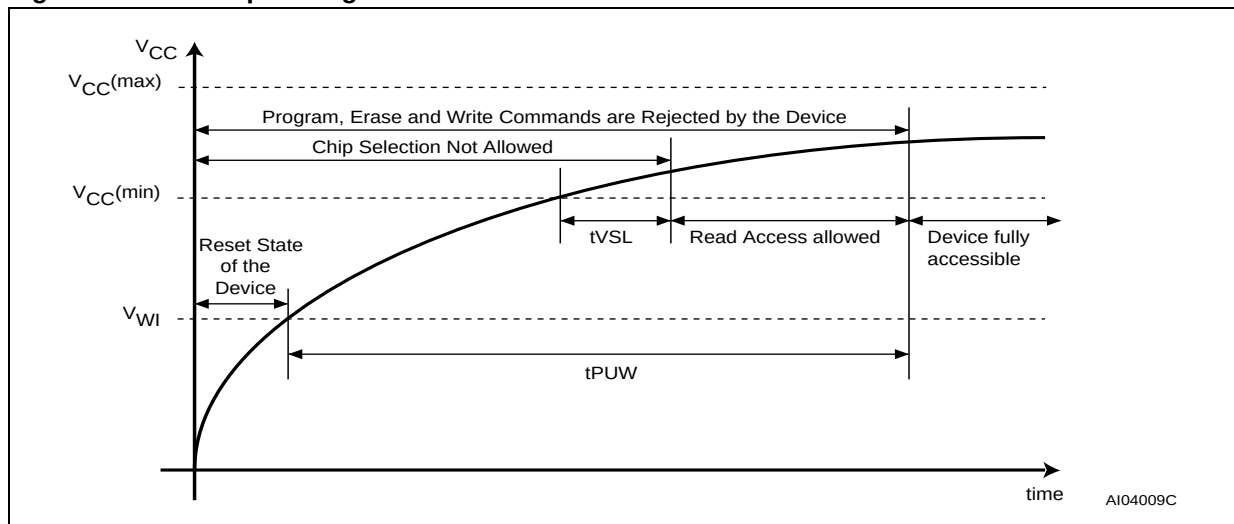
Figure 20. Power-up Timing
