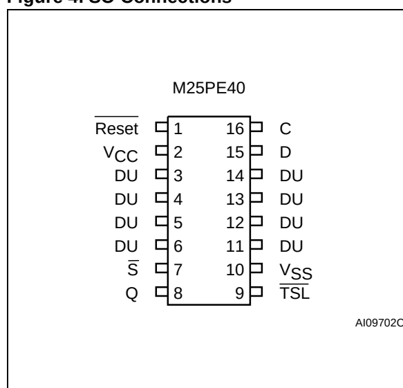
Figure 4. SO Connections
