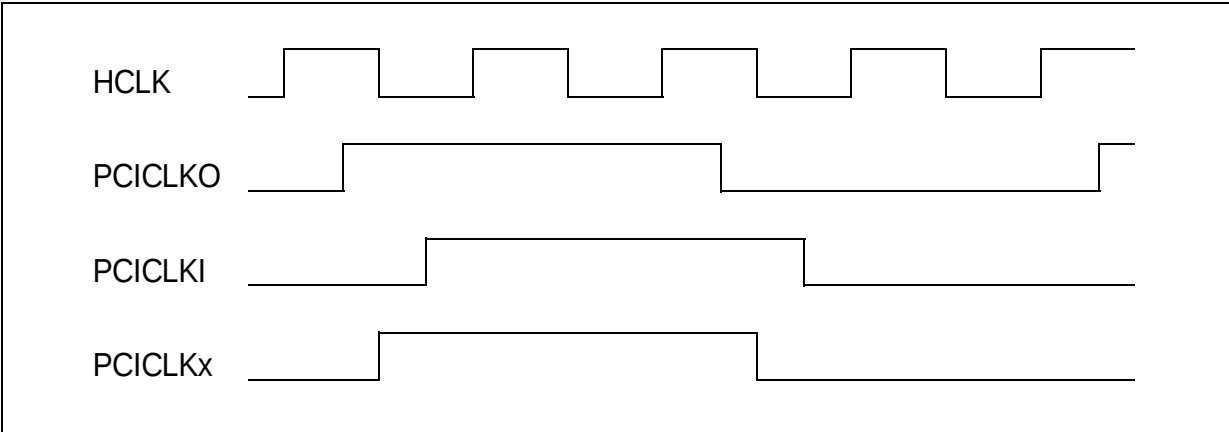
Figure 6-25. Clocks relationships
