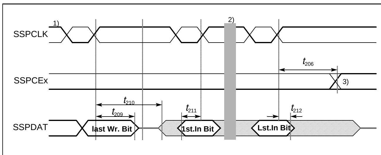
Figure 19 SSP Read Timing
