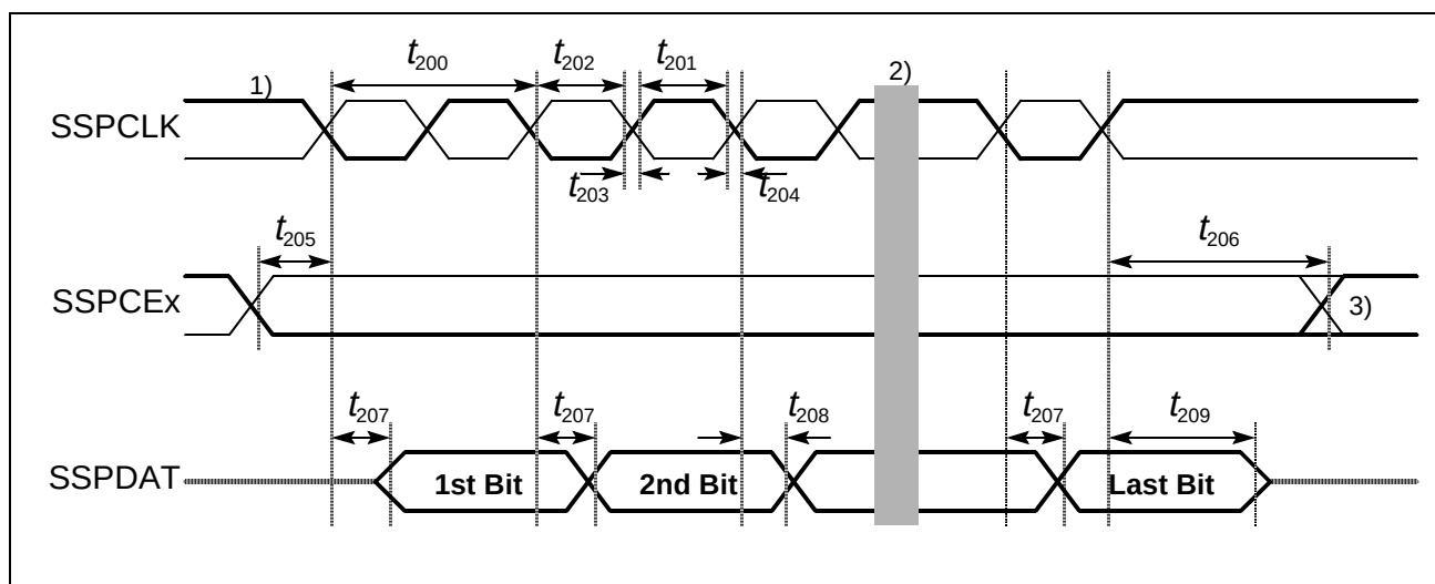
Figure 18 SSP Write Timing
