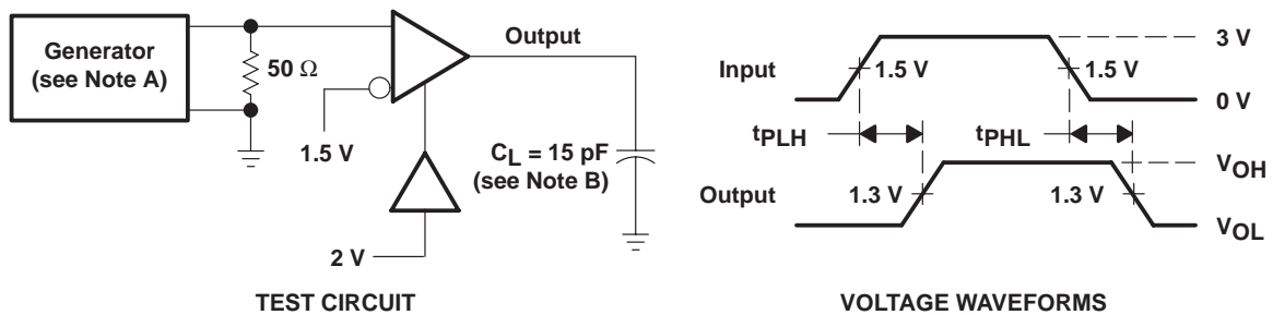
Figure 1. V_{OH} , V_{OL}
