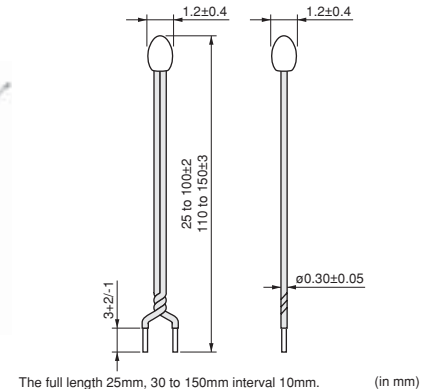
NXFT15_1B Type(twist)
