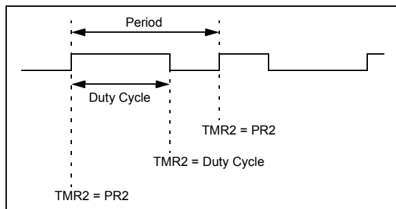
FIGURE 16-4: PWM OUTPUT
