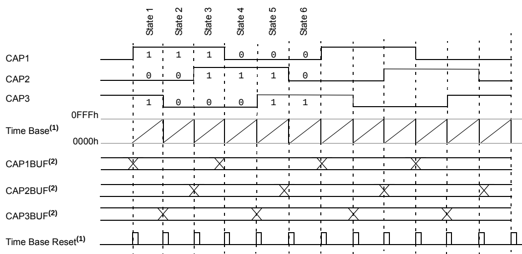
FIGURE 17-6: INPUT CAPTURE ON STATE CHANGE (HALL EFFECT SENSOR MODE)
