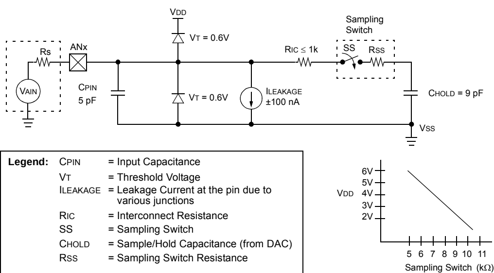
FIGURE 21-2: ANALOG INPUT MODEL
