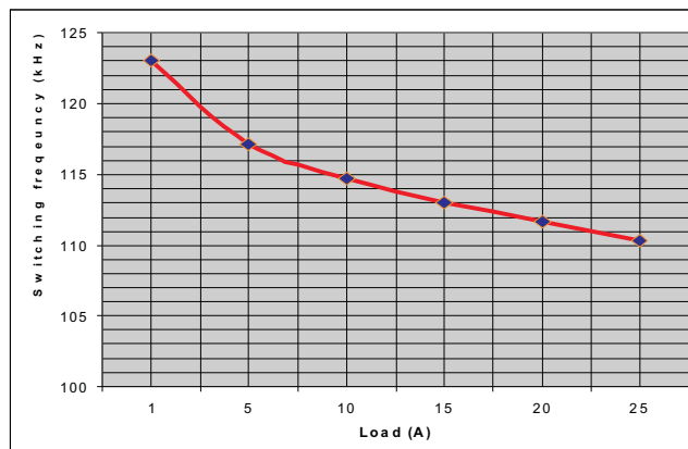
Figure 17. Switching Frequency Variation with Respect to Load (TP24)
