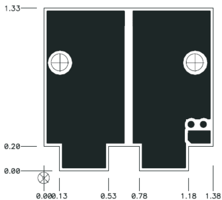
Figure 25. Bottom Copper
