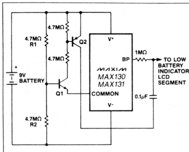
Figure 8. Low Battery Detector and LCD Segment Drive
