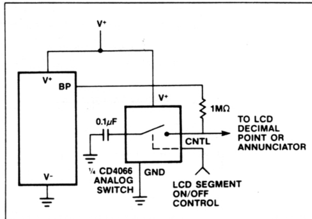
Figure 6D. Analog Switch for Decimal Point Drive
