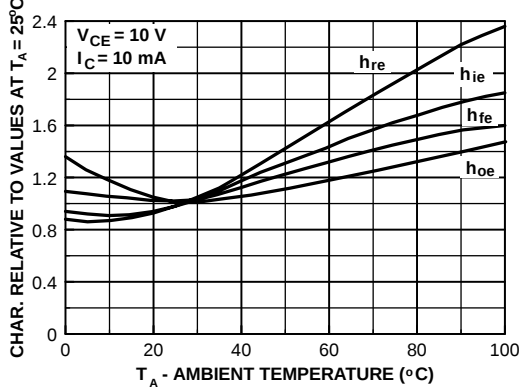
Figure 5. Common Emitter Characteristics
