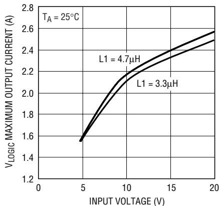
Maximum Output Current for V_{LOGIC} = 3.3\text{V}
