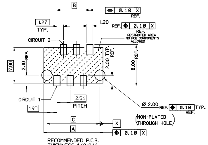
RECOMMENDED P.C.B. THICKNESS 1.60±0.14 PCB LAYOUT FOR CLEARANCE FIT WITH PCB PEGS HEADER VERSIONS 90814-0002-899, VIEWED FROM COMPONENT SIDE
