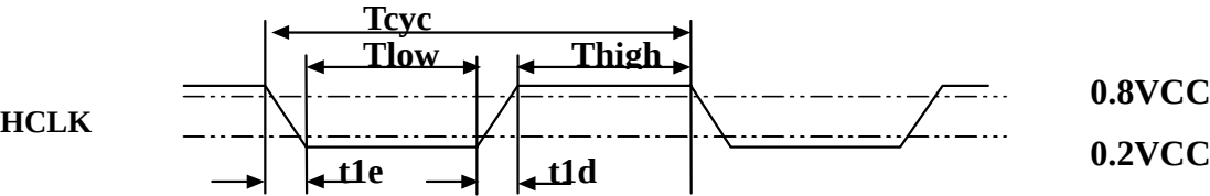
HCLK Timing
