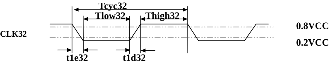
CLK32 Timing
