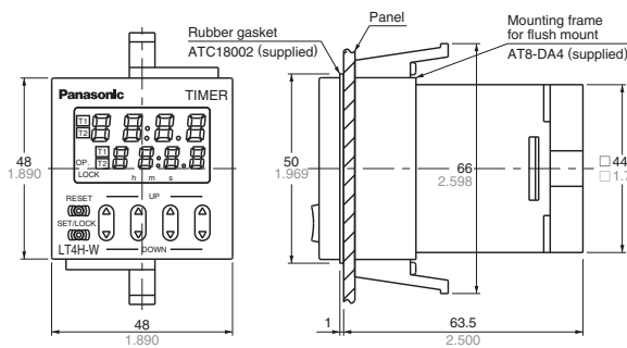
Screw terminal type
